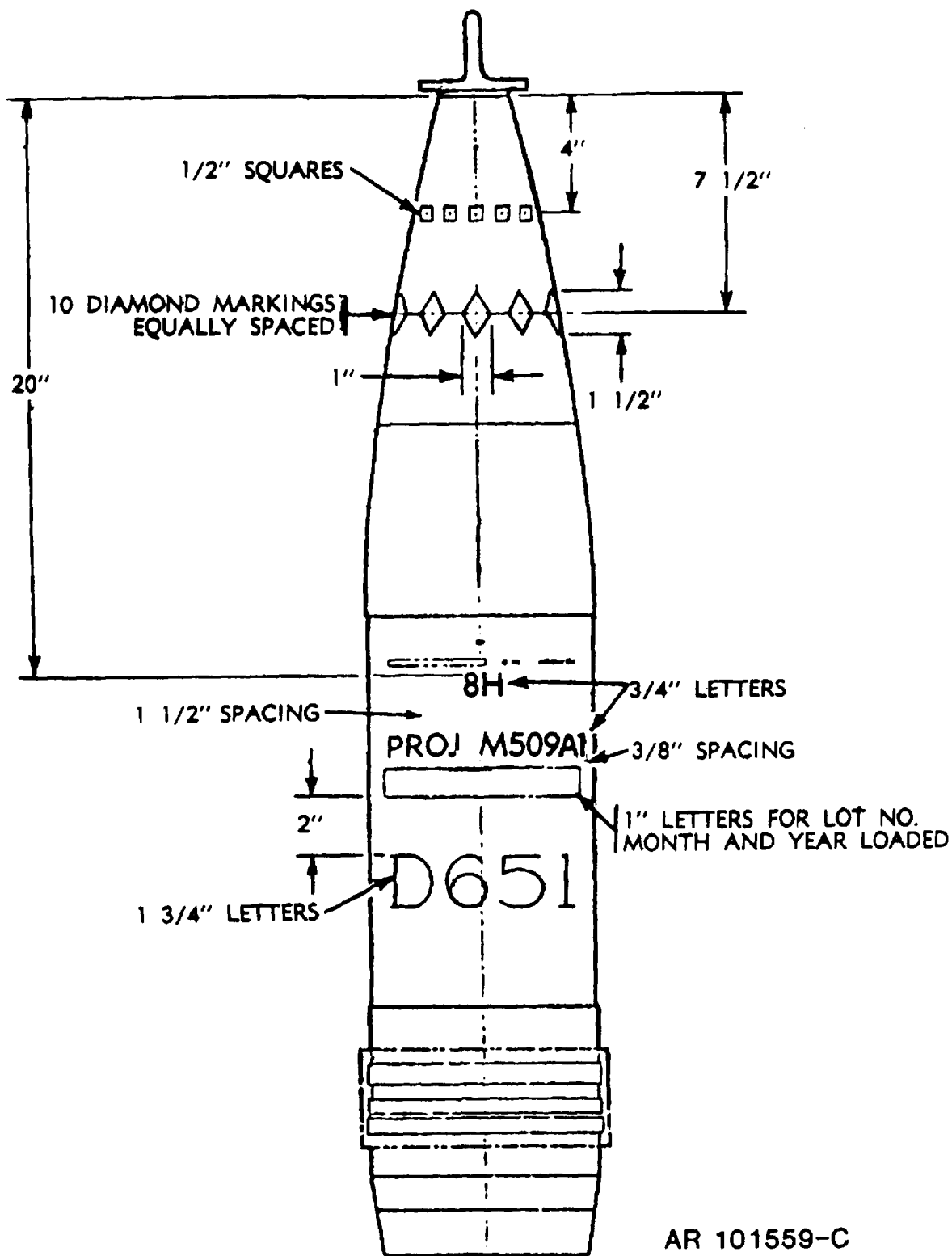
Figure E-101. Typical marking for 8-inch howitzer projectile M509A1.
